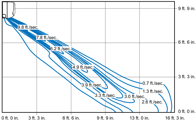
VWMB030H4 - COOLING
