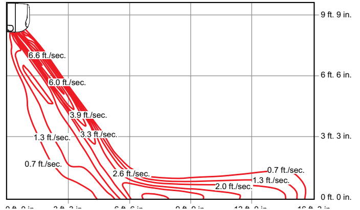
VWMB030H4 - HEATING
