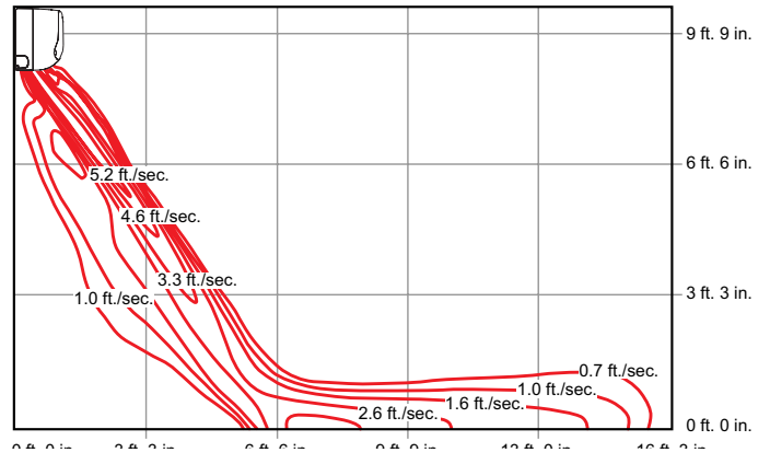
VWMB030H4 - HEATING
