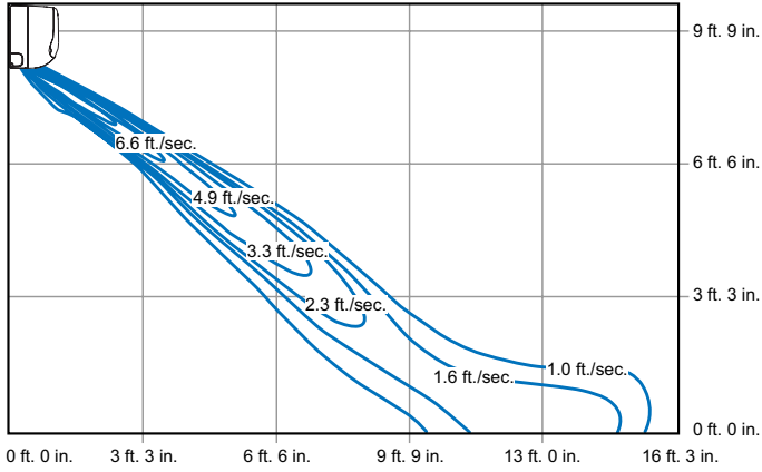
VWMB030H4 - COOLING
