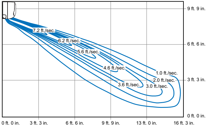
VWMB024H4 - COOLING
