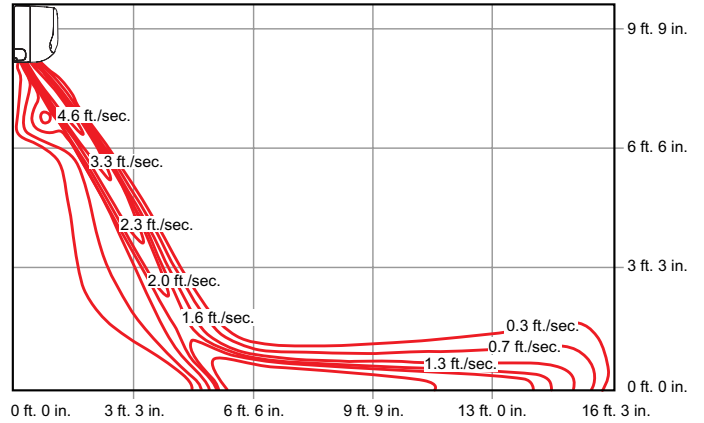
VWMB024H4 - HEATING
